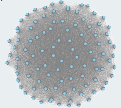
(f) Complete graph n=100
